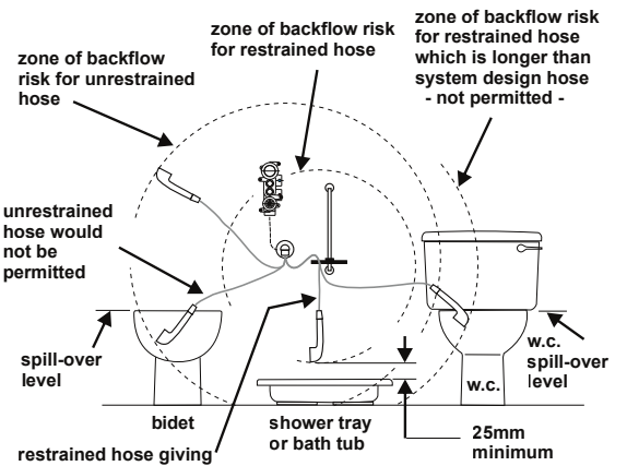
Fig. 4 Backflow risk from a fluid category 5
