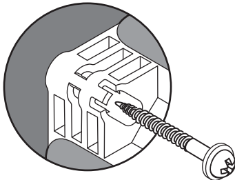
Illustrated above, valve-box being mounted onto a pair of slim noggins (30mm*) attached to the back of a pair of studs. Framework shown here uses 75x50 timbers on 400 centres. (Wall cavity = 75mm).
