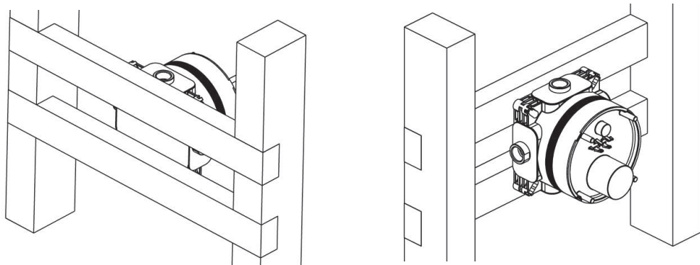
Illustrated above, valve-box being mounted onto a pair of slim noggins (30mm*) attached to the back of a pair of studs. Framework shown here uses 75x50 timbers on 400 centres. (Wall cavity = 75mm).
